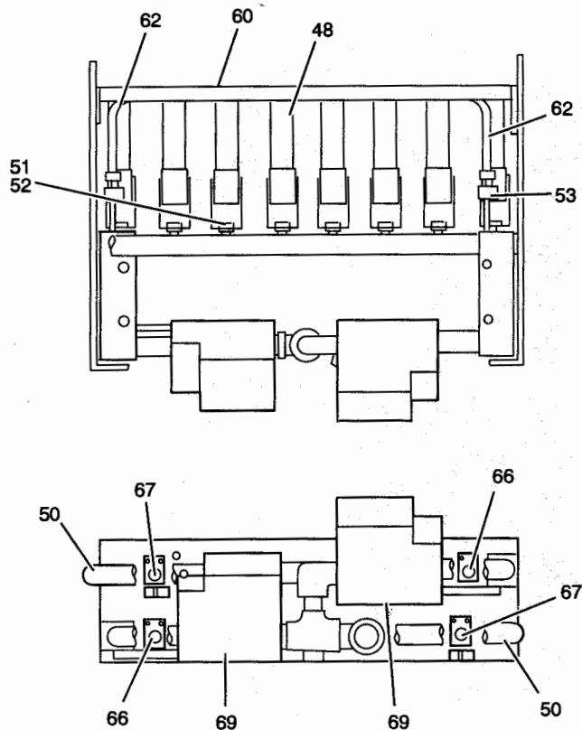
FIG. 5 - BURNER ASSEMBLY
