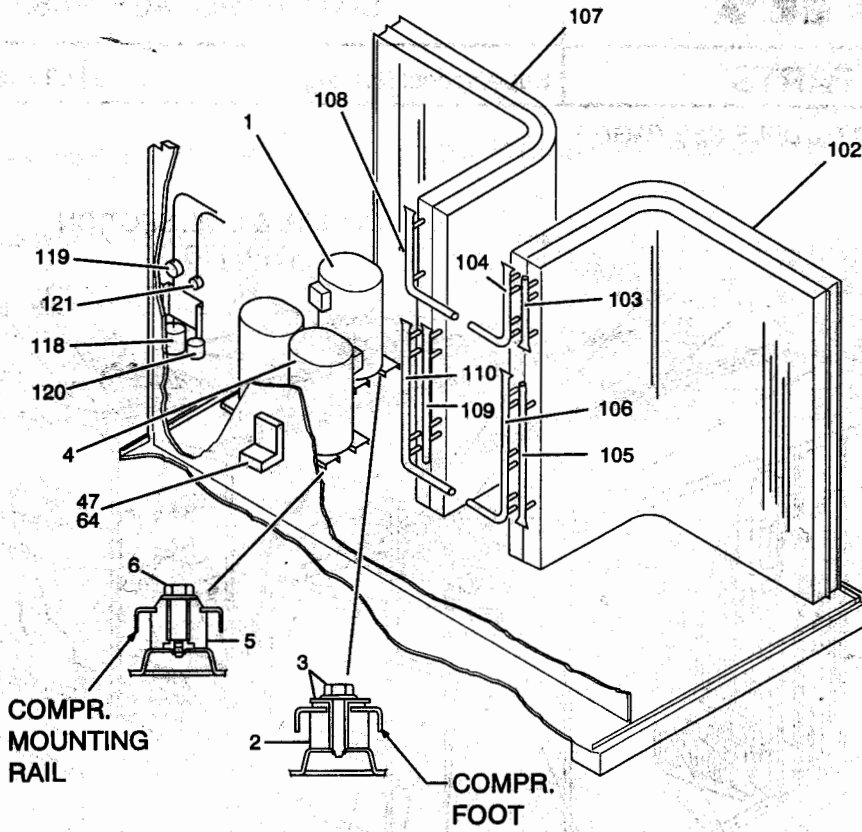
FIG. 2 - COMPRESSOR & COIL SECTION
