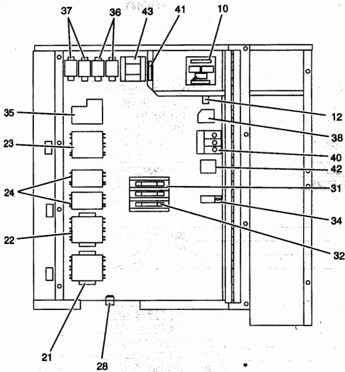
FIG. 3 - ELECTRICAL BOX
